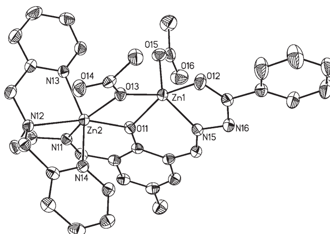
Figure 1. Molecular structure of ZnZn (one of three crystallographically independent molecules shown). Thermal ellipsoids are drawn at the 50% probability level. Hydrogen atoms and non-coordinated solvent molecules are omitted for clarity.
