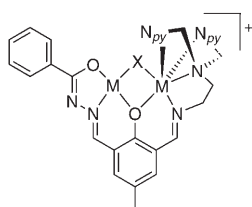
Scheme 3. Formula of the [MM(\text{bpampbh})(\mu\text{-X})]^+ ions found in ESI mass spectra ( M = \text{Ni} and \text{Zn} ).
