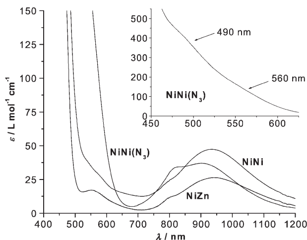
Figure 7. Electronic spectra of complexes \text{NiZn} , \text{NiNi} , and \text{NiNi}(\text{N}_3) at 20°C in acetonitrile ( 2 \times 10^{-3} \text{ M} ).
