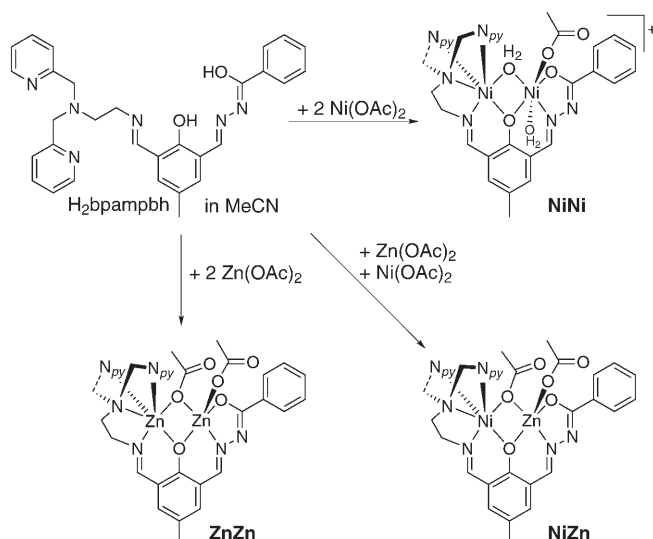
Scheme 2. Synthesis of homo- and heterobimetallic complexes utilizing the unsymmetric double-Schiff-base ligands H_2bpampbh .
