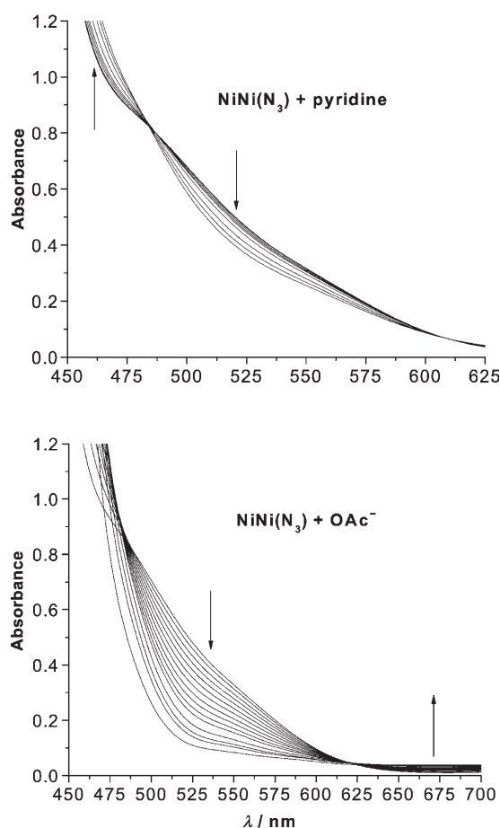
Figure 11. Photometric titration of NiNi(N 3 ) in acetonitrile (2 mm) at 20 °C. Top: Addition of pyridine (0, 0.1, 0.3, 0.5, 0.7, 1.2, 2.2, 3.2, and 4.2 equivalents); Bottom: Addition of tetra- n -butylammonium acetate (0, 0.1, 0.2, 0.3, 0.4, 0.5, 0.6, 0.7, 0.8, 0.9, 1.0, 1.2, 1.4, 1.6, 2.1 equivalents); Absorbance data were corrected for dilution effects.
